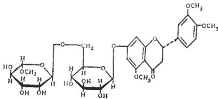
Methylhesperidin
