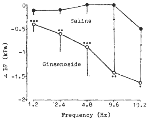
Fig 2. Effect of ginsenosides on pressor response induced by spinal electrical stimulation in pithed rats. \bar{x} \pm SD . * p > 0.05 , ** p < 0.05 , *** p < 0.01
