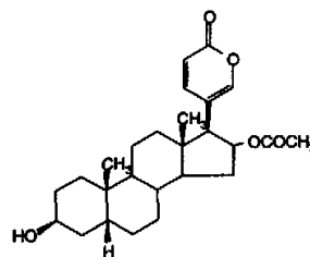
Bufotalin
