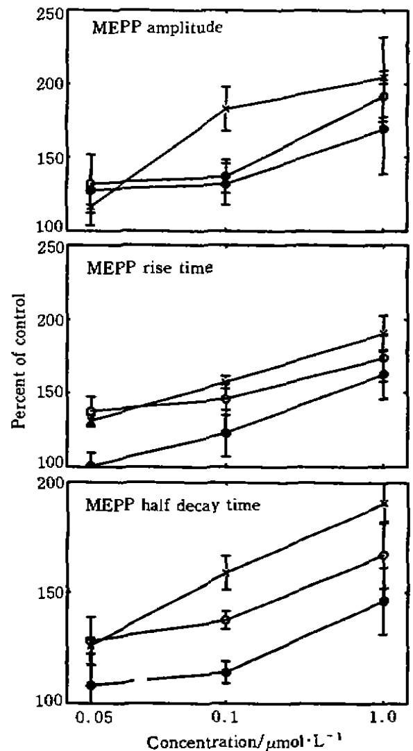
Fig 1. Effects of huperzine-A (O), tacrine (●), and E2020 (x) on MEPP amplitude, rise time, and half decay time. n = 3 preparations, \bar{x} \pm s .
